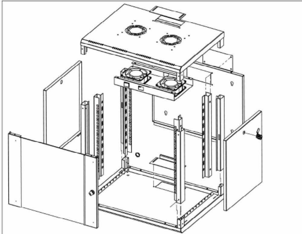
Explode View
