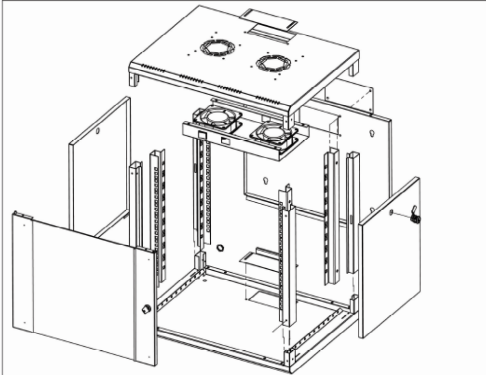
Explode View
